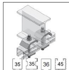
Girder connection horizontal Page 2/56
